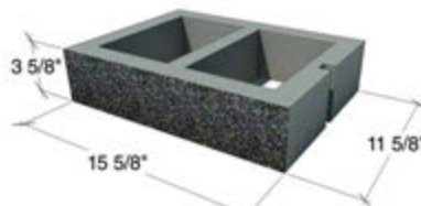
12x4x16 SASH - SP1S, G1S, SMO
