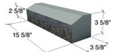
4x4x16 SOLID SLOPED SILL - SP1S, G1S OR SMO (SLOPED FACE G OR SMO)
