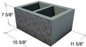
12x8x16 HOLLOW - SP1S, G1S, SMO
