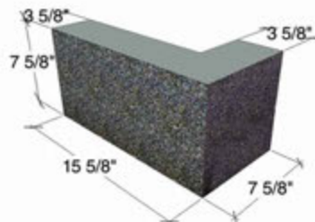
4x8x16 SOLID L-CORNER - SPC, G1S1E OR SMO
