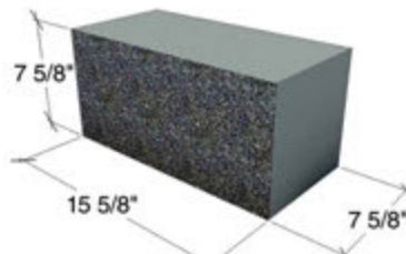
8x8x16 SOLID - SP1S, G1S, SMO
