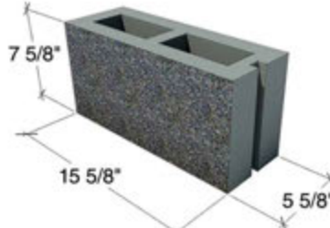
6x8x16 SASH 1S1F - SP1S, G1S, SMO
