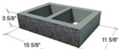
12x4x16 HALF HIGH - SP1S, G1S, SMO
