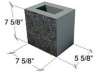
6x8x8 HALF - SP1S, G1S, SMO
