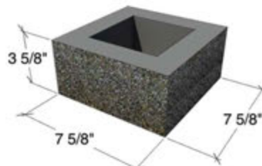
8x4x8 CORNER - SPC, G1S1E, SMO
