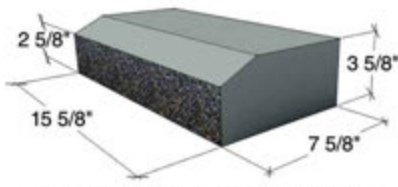
8x4x16 SOLID SLOPED SILL - SP1S, G1S OR SMO (SLOPED FACE G OR SMO)
