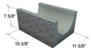
12x8x16 SOLID BOTTOM BB - SP1S, G1S, SMO
