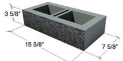
8x4x16 SPITTABLE - SPC, G1S1E, SMO
