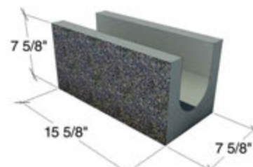
8x8x16 SOLID BOTTOM BB - SP1S, G1S, SMO
