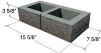
8x4x16 1S1F CORNER - SP1S, G1S, SMO
