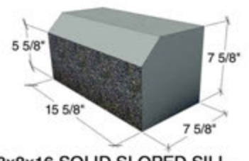
8x8x16 SOLID SLOPED SILL - SP1S, G1S OR SMO (SLOPED FACE G OR SMO)
